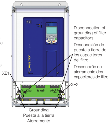
Figure A.6: Grounding points and the location of filter capacitors ground disconnection points - disconnection trough bolts
